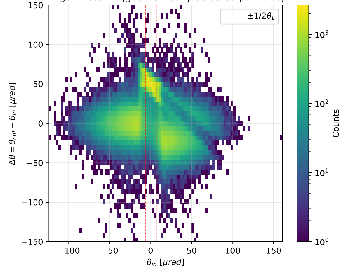
Angular scan - (geometrically selected particles)
