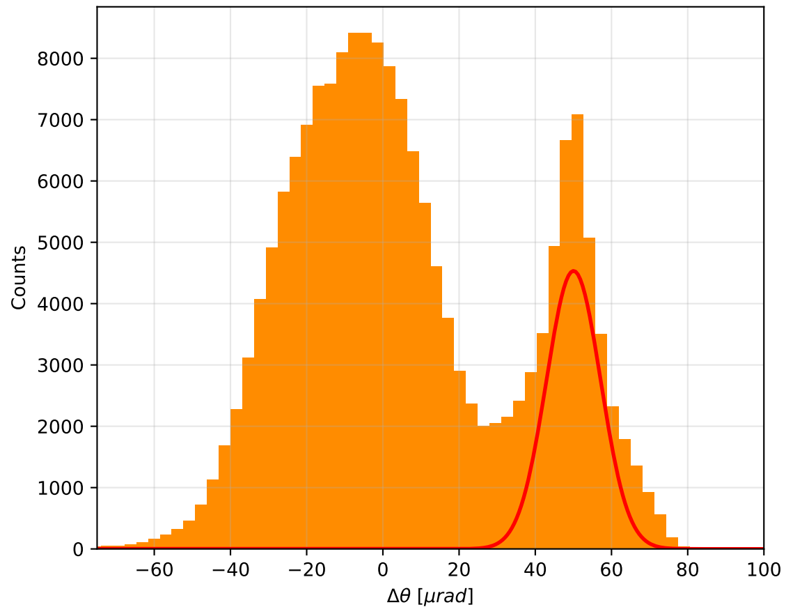
\Delta\theta distribution - (geometrically selected particles)
